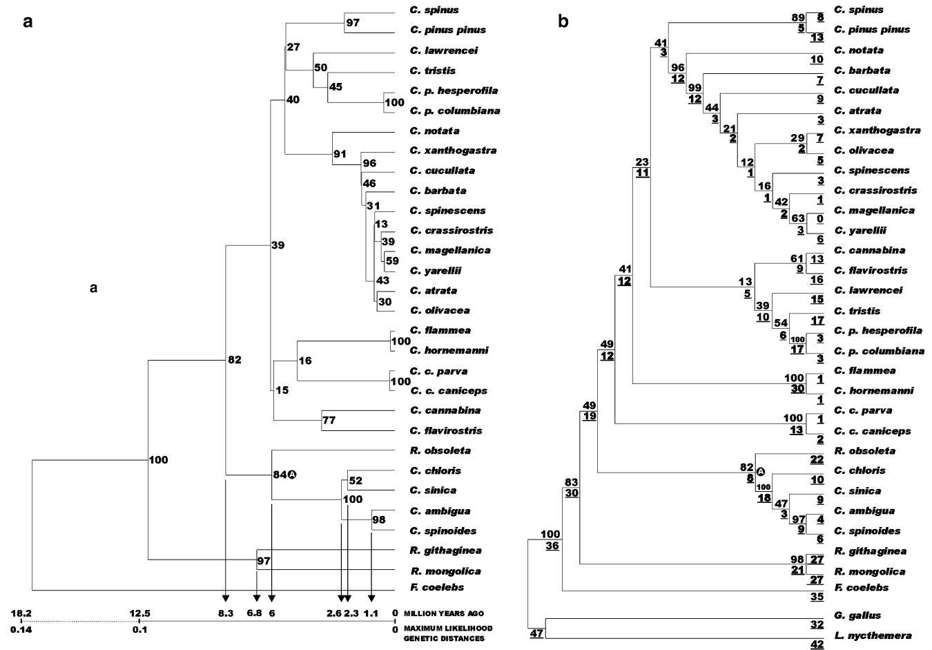
Fig. 1 a Maximum likelihood-based tree showing approximate calculations on the time of appearance of genera Carduelis and Rhodepechys lineages. This linearized tree was constructed by assuming that evolutionary rates between lineages may be different (Thorne et al. 1998). PARAMCLOCK PAUP command was used for tree building. Divergence times were estimated assuming an evolutionary rate of 0.8% substitutions per site and per million years, found by Fleischer et al. (1998). This rate is based on the cyt b sequence divergence of Hawaiian drepanidines, and external geological calibration points. Groups of taxa are similar to those obtained in the parsimony (see b ) and NJ with ML genetic distance dendrograms (tree not shown). Genus Carduelis speciation seems to have occurred during the Miocene and Pliocene epochs in both the Northern and Southern Hemispheres (Arnaiz-Villena et al. 1998). R. mongolica and R. githaginea cluster separately from R. obsoleta , which appears as the greenfinch ancestor. One thousand replication bootstrap values are depicted in the interior part of the nodes. ML-based tree scores: tree length (1,000 times) = 1,055; ln
