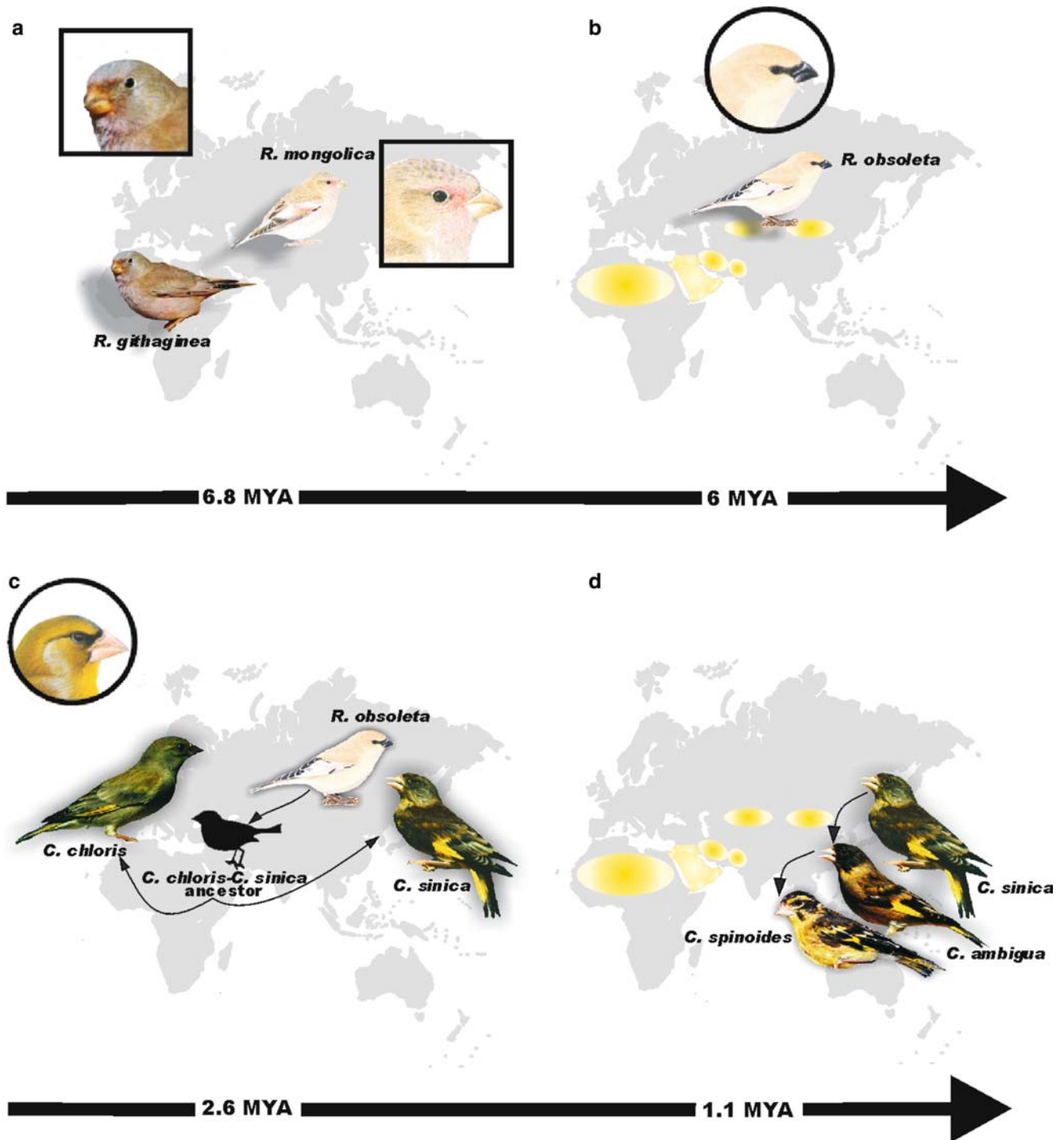
Fig. 2 Hypothetic model of greenfinch group evolution from semi-desert land based populations of R. obsoleta . Birds are placed approximately over their present distribution areas. Approximated times in million years for each dispersion are in accordance to Fig. 1a: a Molecular unrelatedness of R. githaginea and R. mongolica ; b Apparition of R. obsoleta in desert areas (yellow); c Postulated dispersion of R. obsoleta populations that would have given rise to a C. chloris - C. sinica ancestor which would have evolved separately to reach different species status; d Postulated
